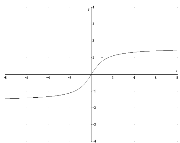
y = \text{arctg } x
