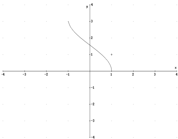
y = \text{arccos } x
